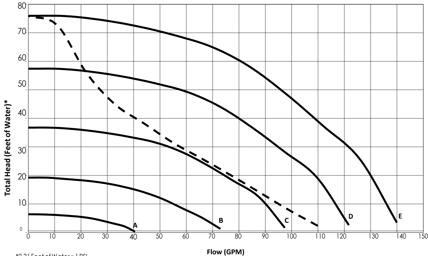
JVS185S - 1.85 THP Variable Speed Pump
